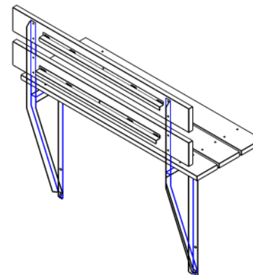
ASSEMBLED VIEW
