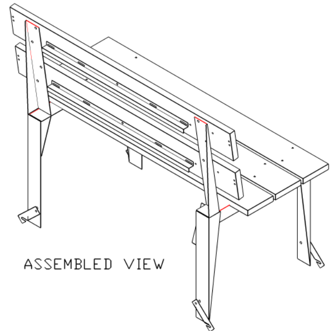
Moveable Bench Frame (Left & Right)
